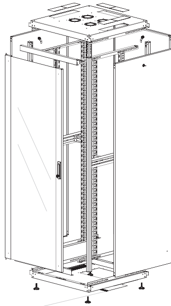
Exploded view
