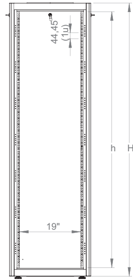
Dimensions in width and height
